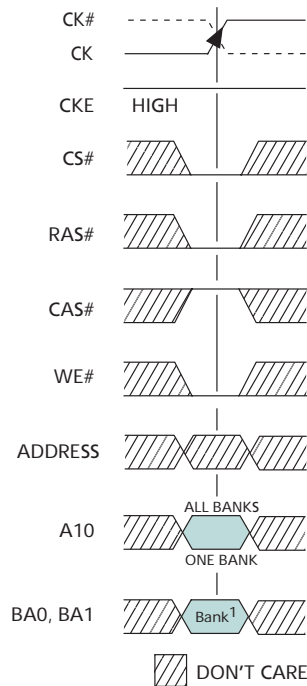
Figure 20: PRECHARGE Command
