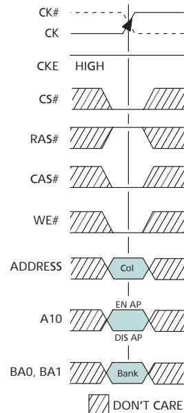
Figure 19: WRITE Command
