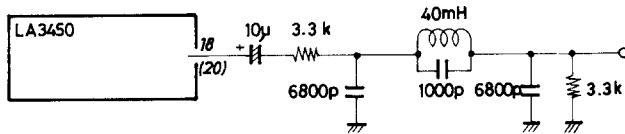
Fig. 5 Sample Circuit of LC Filter
