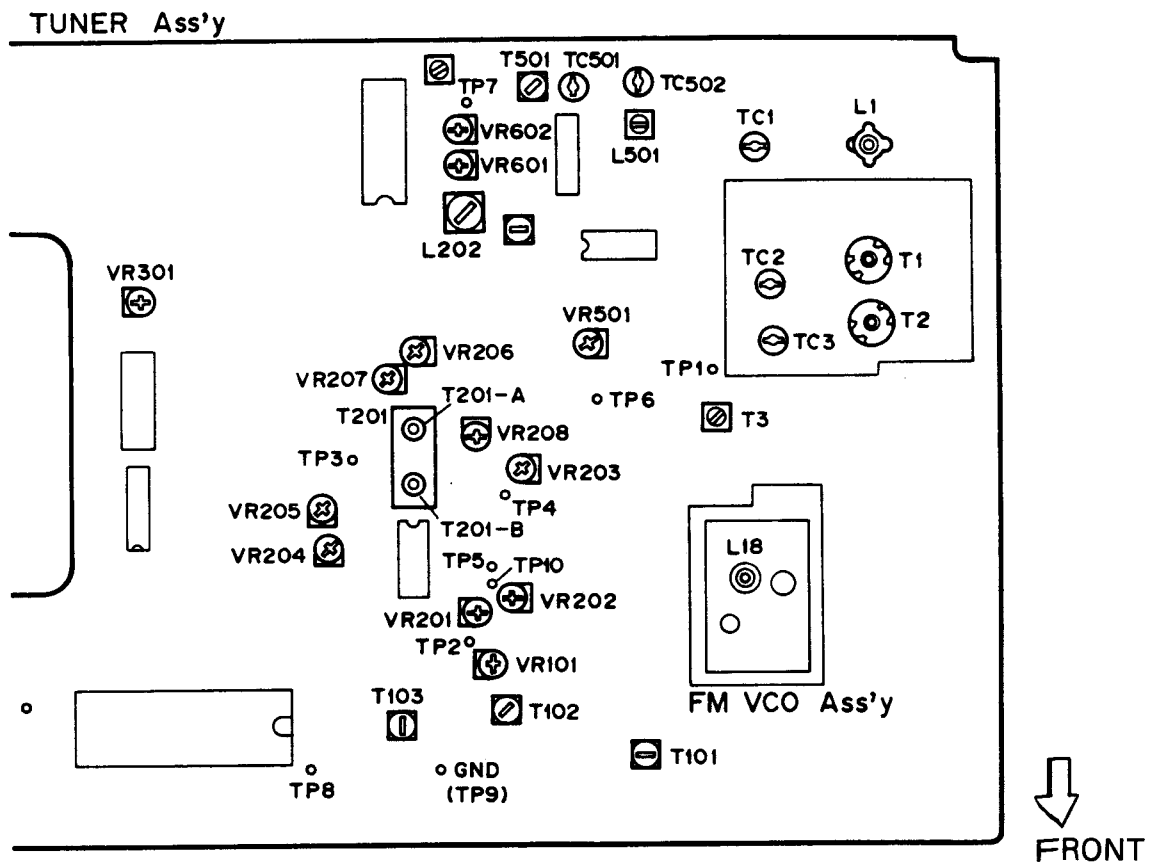
Fig. 6-3 Adjusting point
