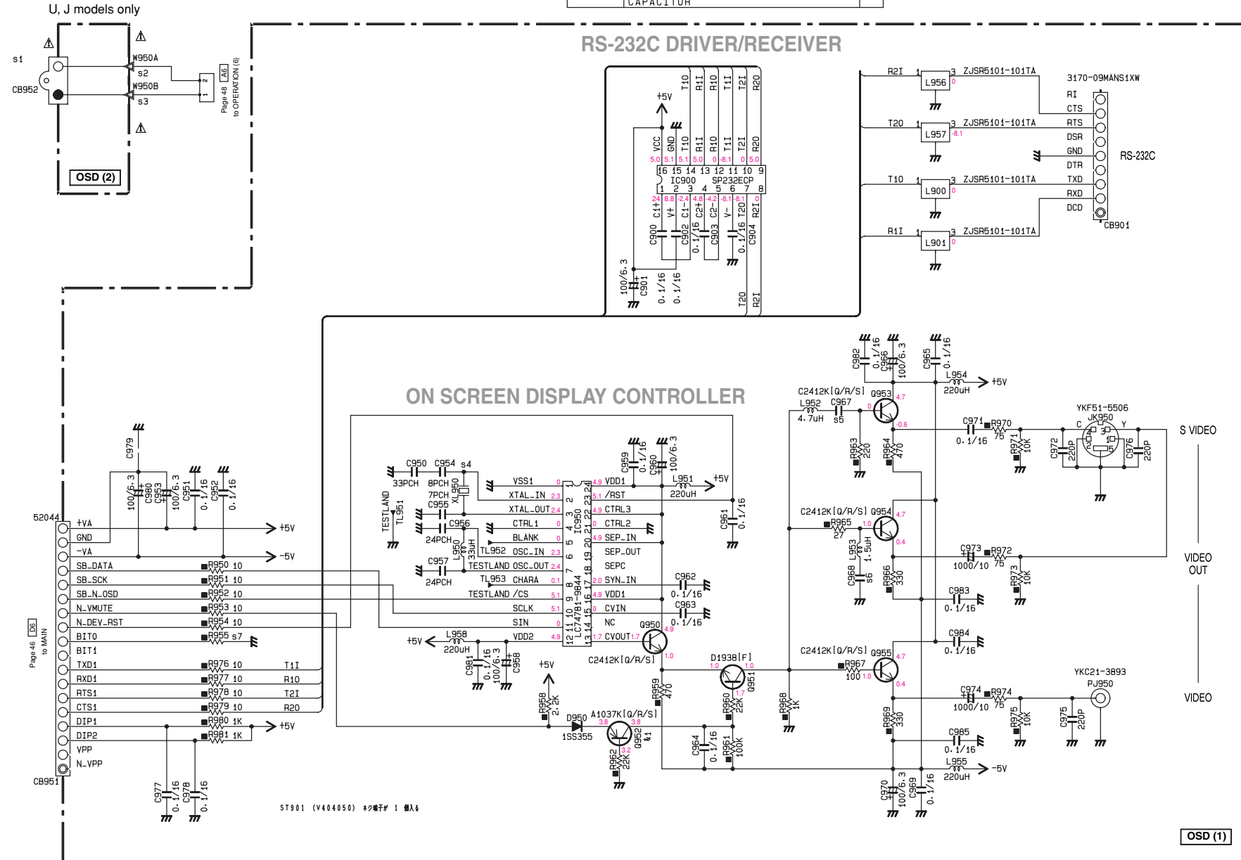
IC900: SP232ECP RS232C Driver/Receiver
