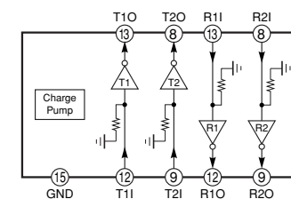
IC900: SP232ECP RS232C Driver/Receiver
